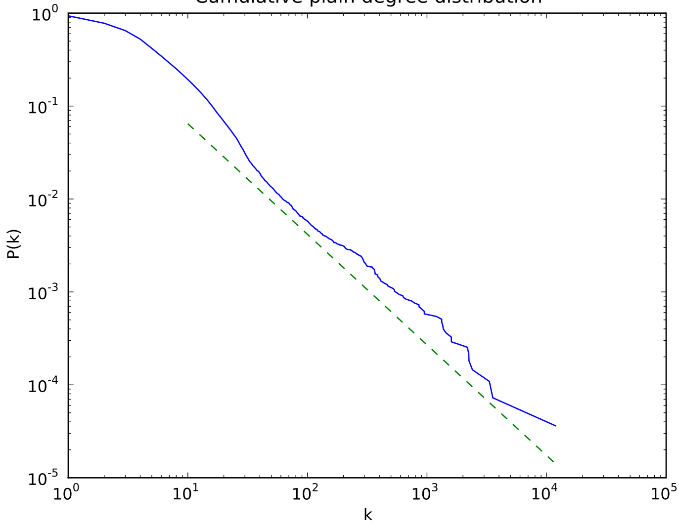
Cumulative plain degree distribution
