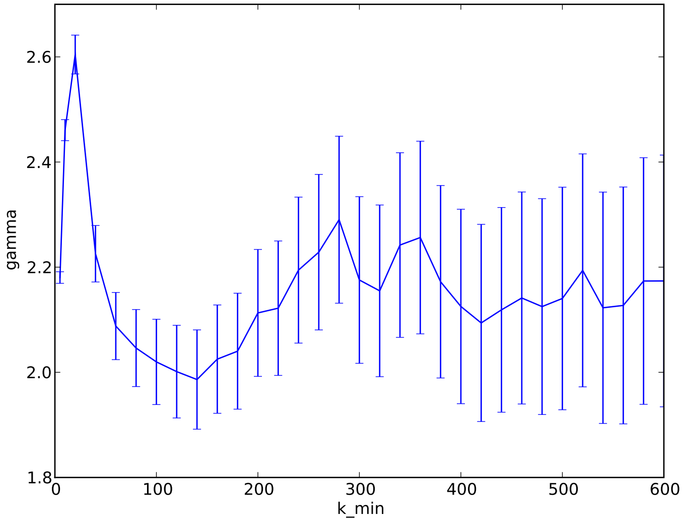
The dependence from k_{\min} of the exponent (plain degree)
